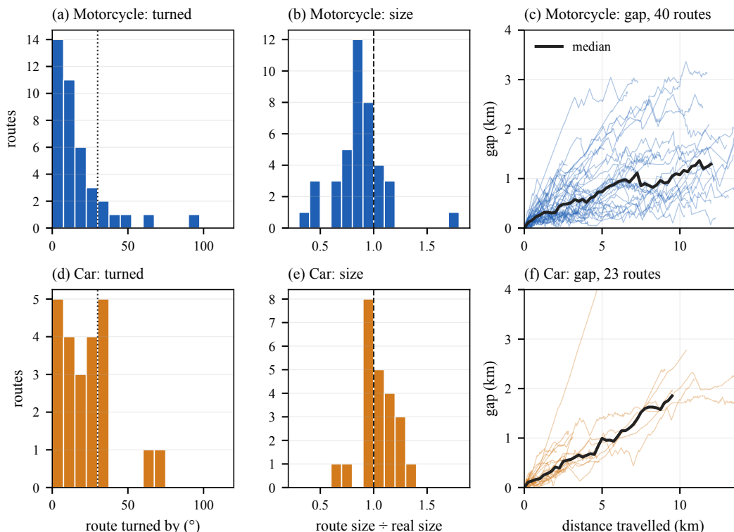
Figure 4: Routes drawn by the app, compared with GPS. (a, d) How far each whole route is turned from the GPS track; the dotted line is 30°. (b, e) Its size relative to the GPS track. (c, f) How far the drawn position is from the GPS position as the journey goes on: one thin line per route, and the median.
